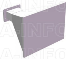
LB-430-15-ASPO Standard Gain Horn Antenna 1.7-2.6GHz 15dB Gain Rectangular Waveguide Interface
