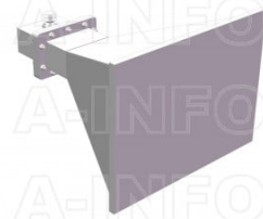
LB-430-15-C-7/16FSPO Standard Gain Horn Antenna 1.7-2.6GHz 15dB Gain 7/16(DIN) Female
