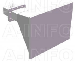
LB-430-15-C-SFSPO Standard Gain Horn Antenna 1.7-2.6GHz 15dB Gain SMA Female
